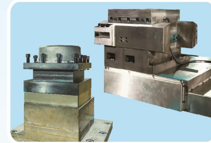
刀架 Turret tool holder
